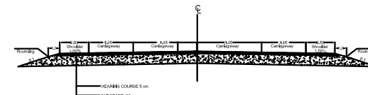
SECTION AT C-C
