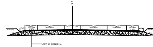
SECTION AT B-B
